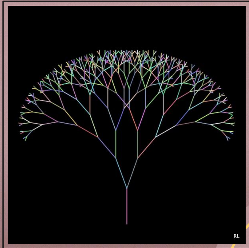
Fractals
