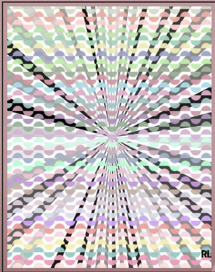
Optical Illusion
